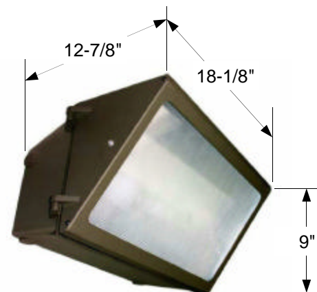
QPE25 Max. 400W MH or 400W HPS
