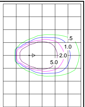
Type IV distribution forward throw.
