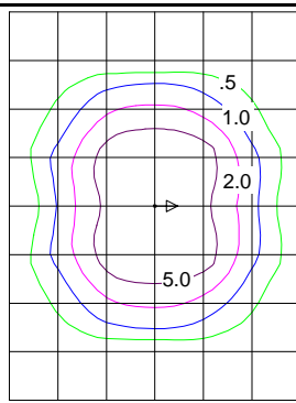
Type II distribution wide throw.
